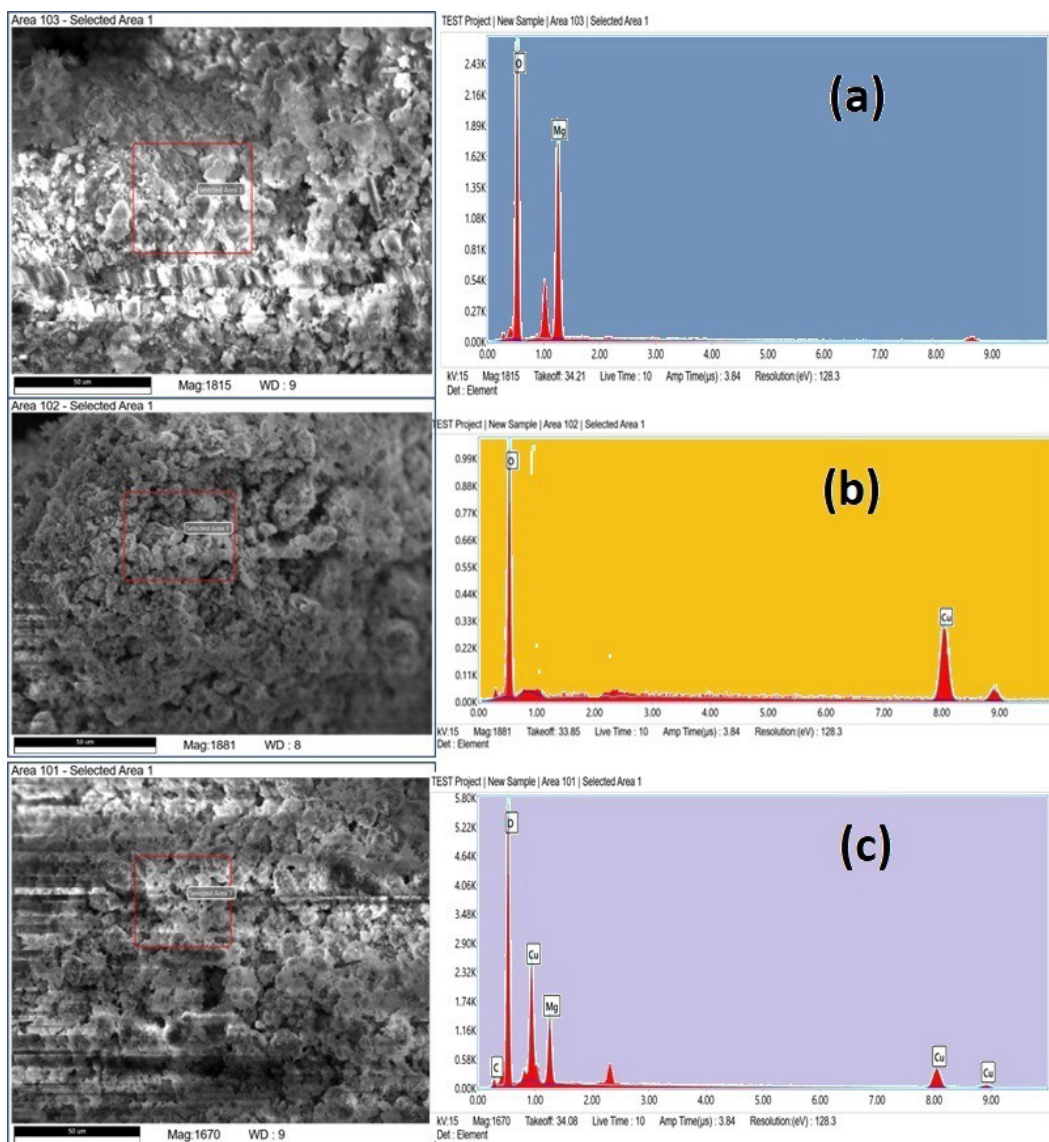
Figure 3. EDX spectra of (a) bulk MgO, (b) CuO-NPs, and (c) the MgO/CuO composite dried at 80°C for 10 h.
