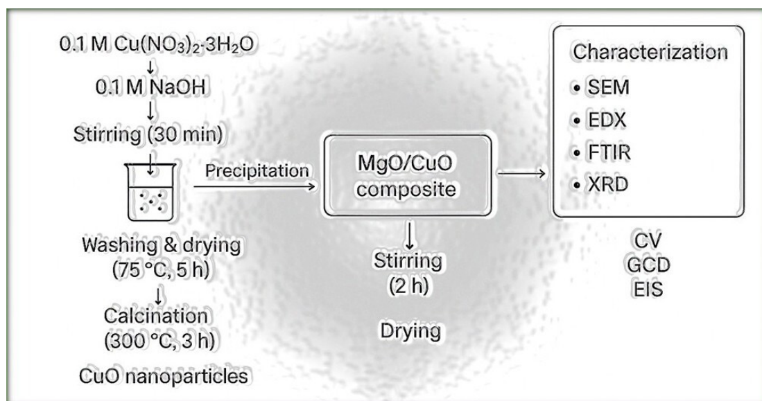
Figure 1. Schematic representation of the synthesis process of the CuO/MgO composite
