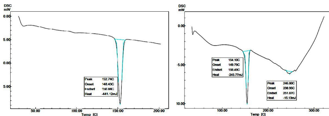
Figure 5. DSC thermograph of the pure drug (a) and optimized batch (b).
