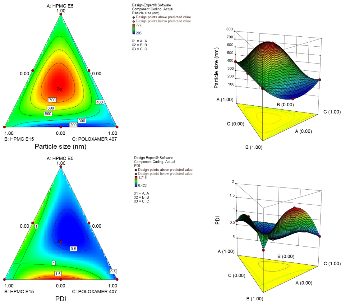
Figure 2. Contour plot and 3-D surface plot depicting the effect of the independent variable on response variable Y_1 (particle size) (a) and contour plot and 3-D surface plot depicting the effect of the independent variable on response variable Y_2 (PDI) (b).
